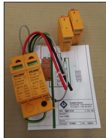
Retrofit Kit; Surge Arrestor with wiring loom, connect diagram, spare cartridges, Order # 313 000 206
