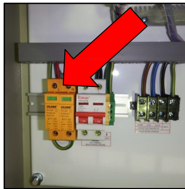
Installed surge arrestor in SD75 Cartridge indicator; Green is good, Red is blown
